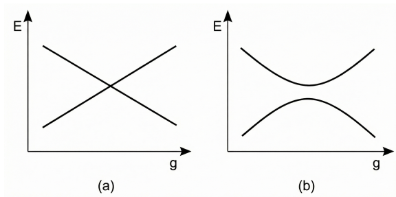
Energy gap closing at a QPT vs. avoided level-crossing.
